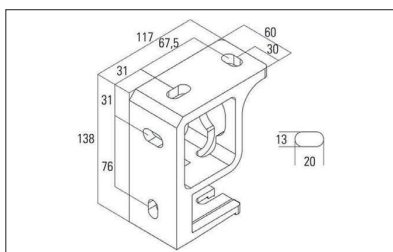
Staffa parete/soffitto Wall/ceiling bracket
