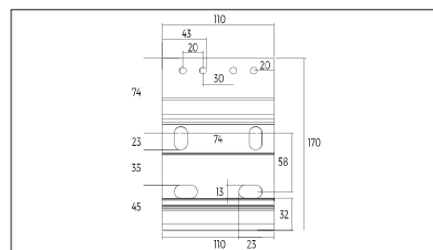
Staffa parete / soffitto Wall / ceiling bracket
