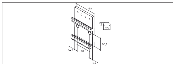
Staffa parete / soffitto Wall / ceiling bracket
